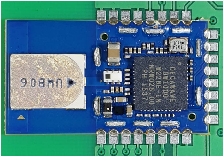
Photo 6: UWB chip, same model
