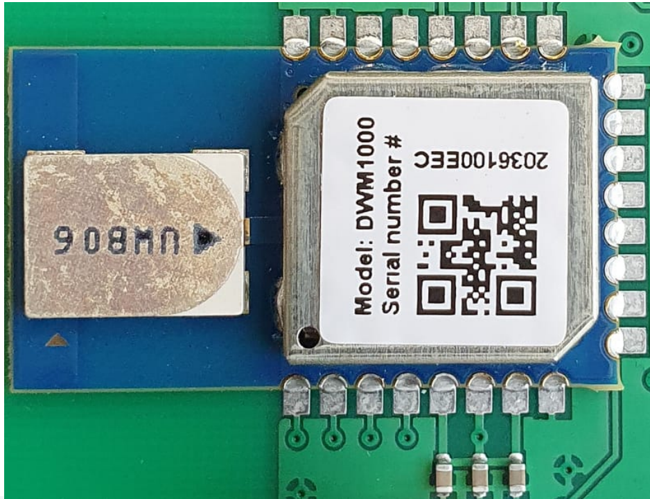
Photo 5: UWB chip, same model
