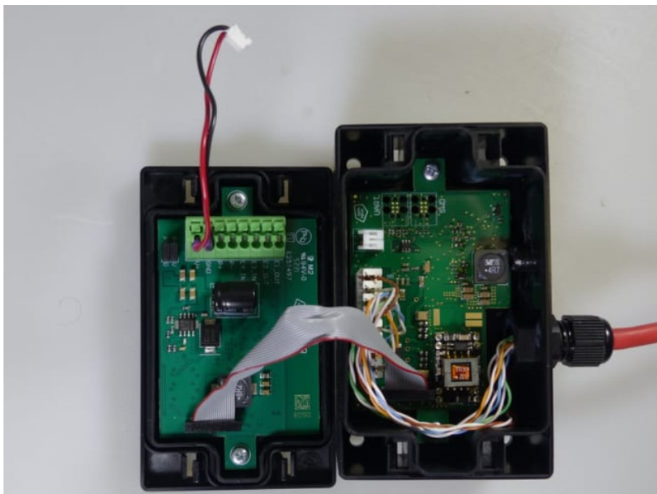
Photo 12: Radio board disconnected, only PoE board active
