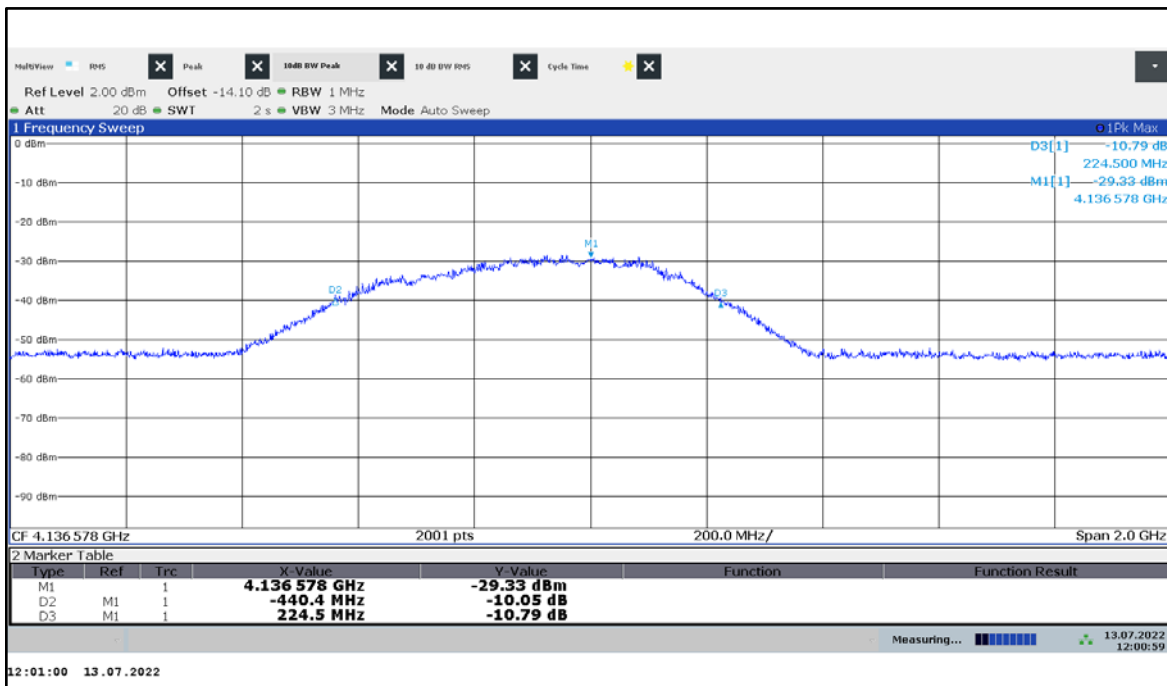
Plot 2: 10 dB bandwidth, UWB test mode channel 2
