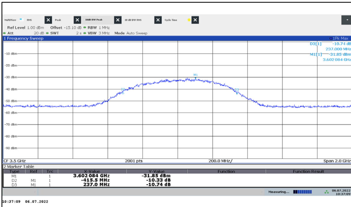
Plot 1: 10 dB bandwidth, UWB test mode channel 1
