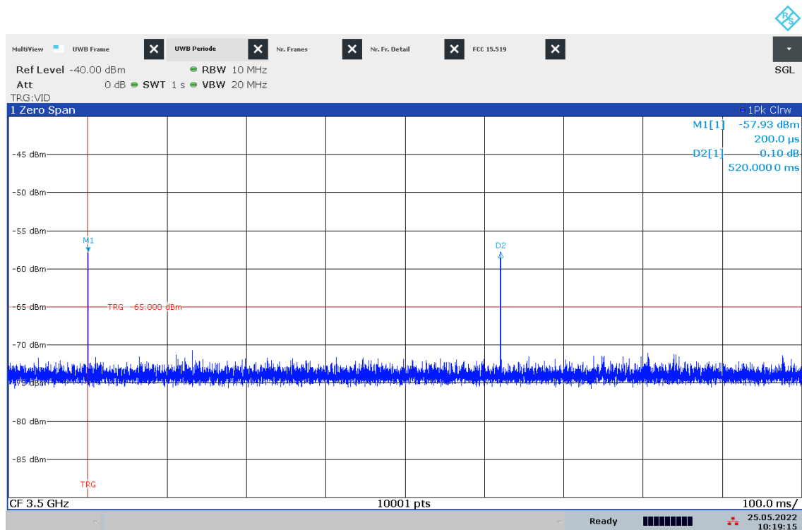
Plot 26: Emission of EUT without associated receiver (for comparison), normal mode Channel 1
