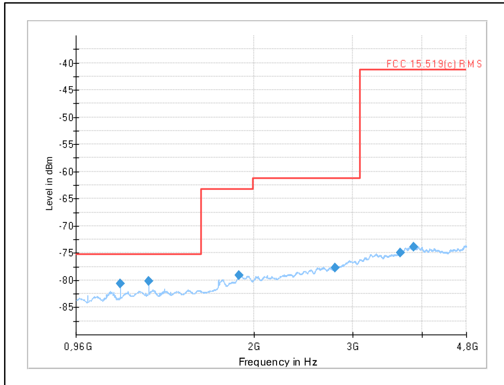
Plot 30: 960 MHz to 4.8 GHz (Limit acc. to §15.519 (c)), UWB test mode
