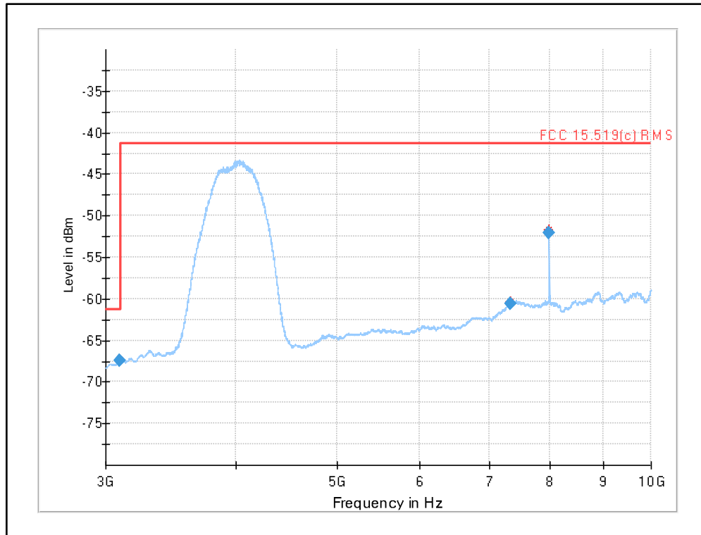
Plot 20: 3.2 GHz to 10 GHz, UWB test mode
