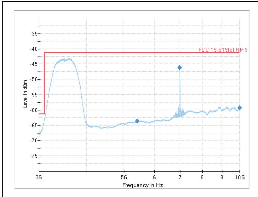
Plot 9: 3.2 GHz to 10 GHz, UWB test mode
