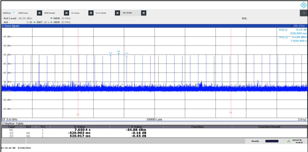
Plot 38: Emission of EUT without associated receiver (for comparison), normal mode
