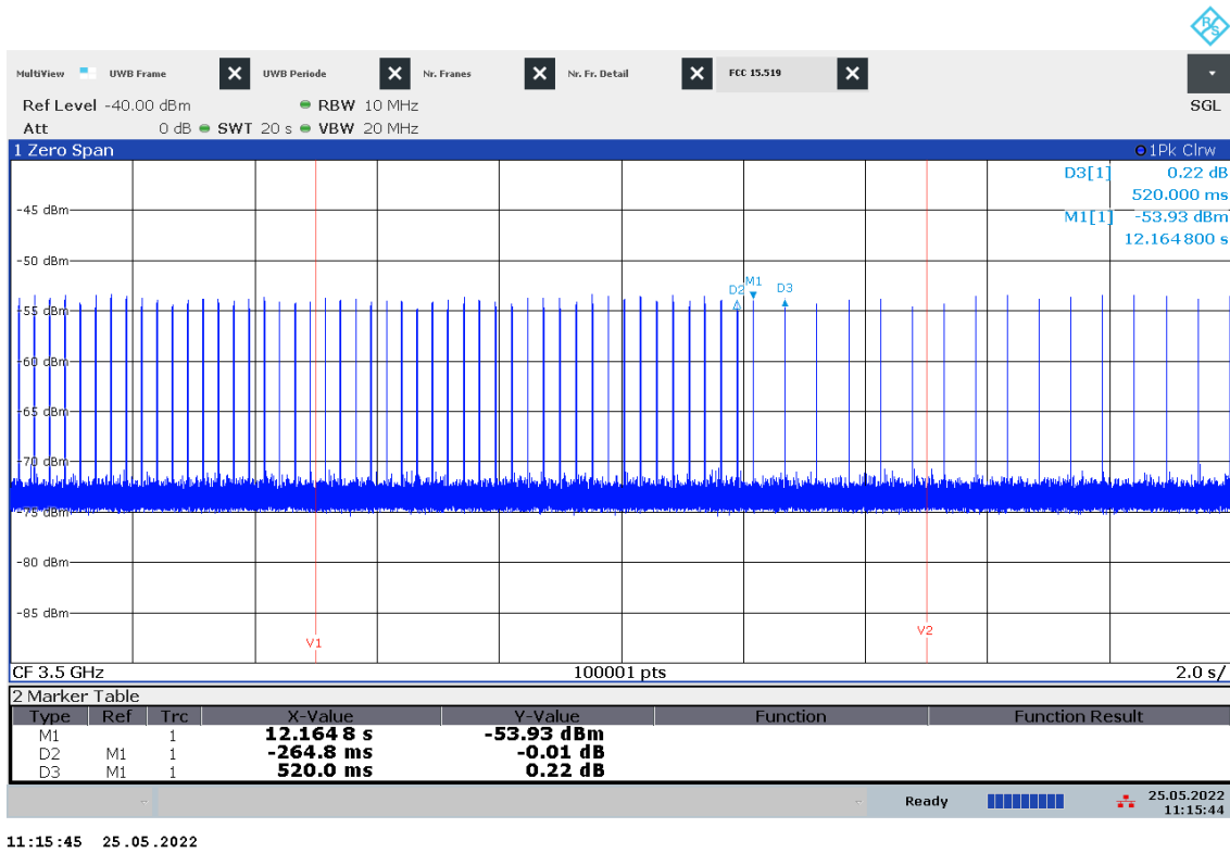
Plot 27: Emissions of the EUT, only at the beginning with associated receiver (Normal mode), Channel 1
