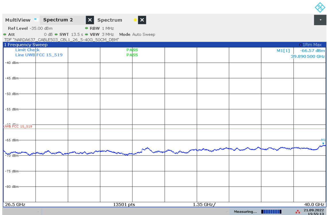
Plot 11: 26.5 GHz to 40.0 GHz, UWB test mode
