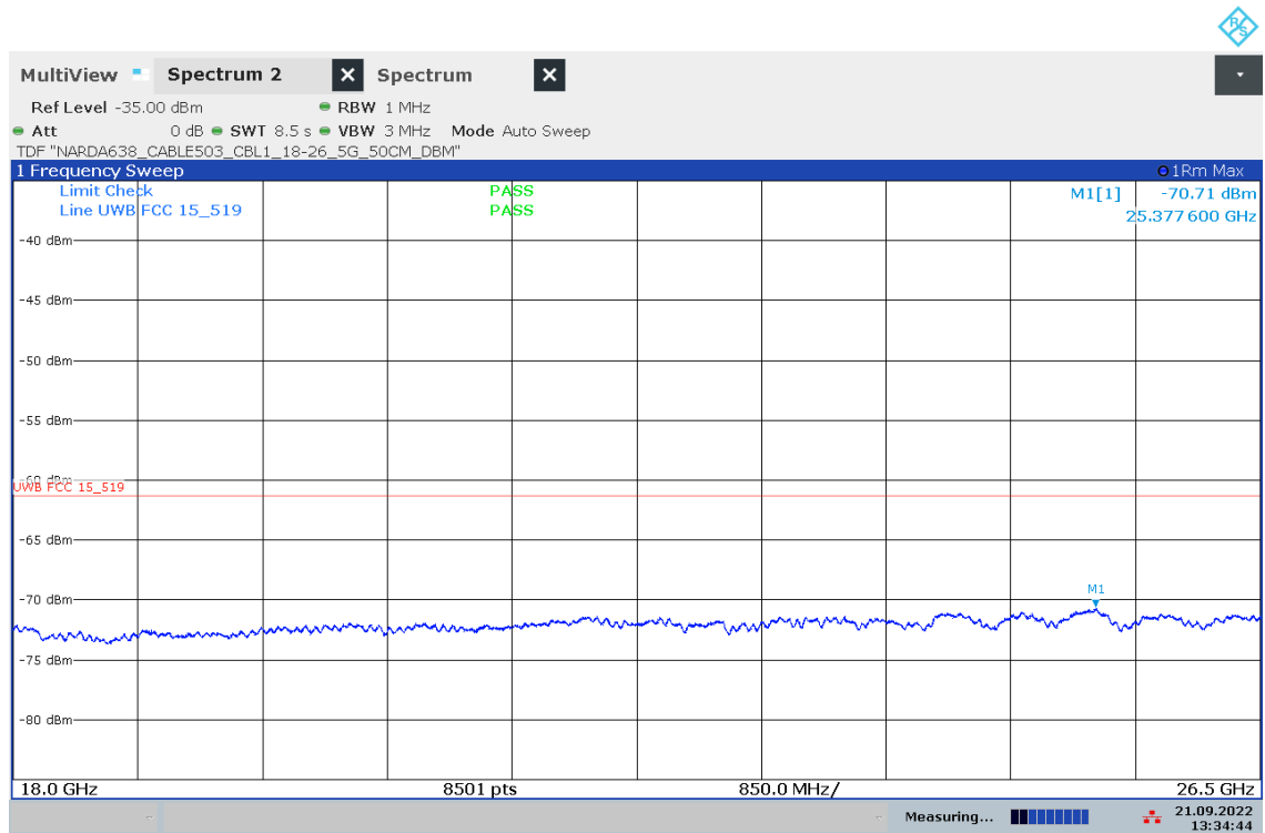
Plot 10: 18 GHz to 26.5 GHz, UWB test mode
