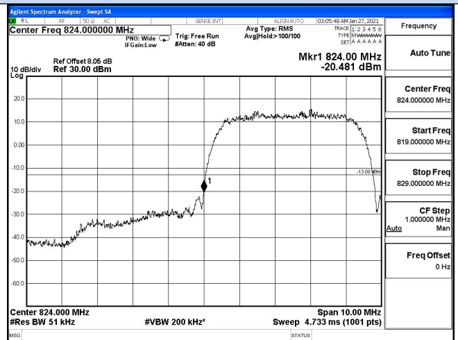
Channel 4132 / 826.4 MHz
