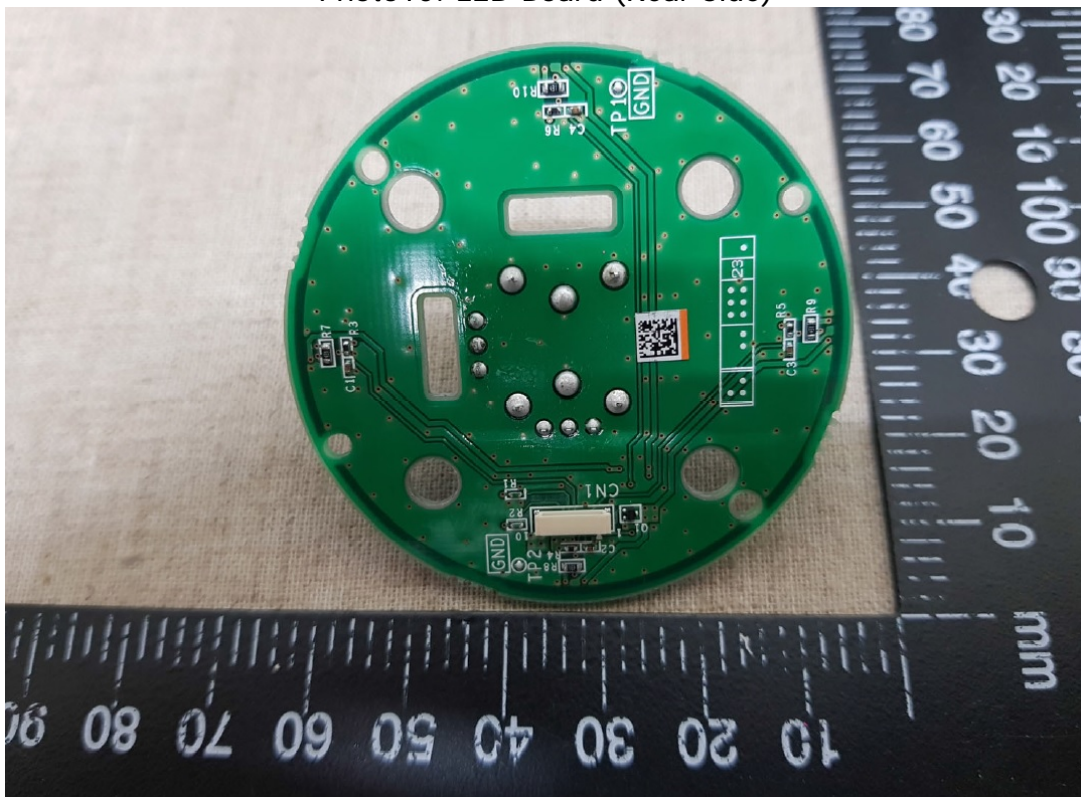
Photo10: LED Board (Rear Side)
