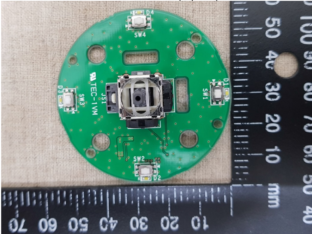
Photo10: LED Board (Rear Side)
