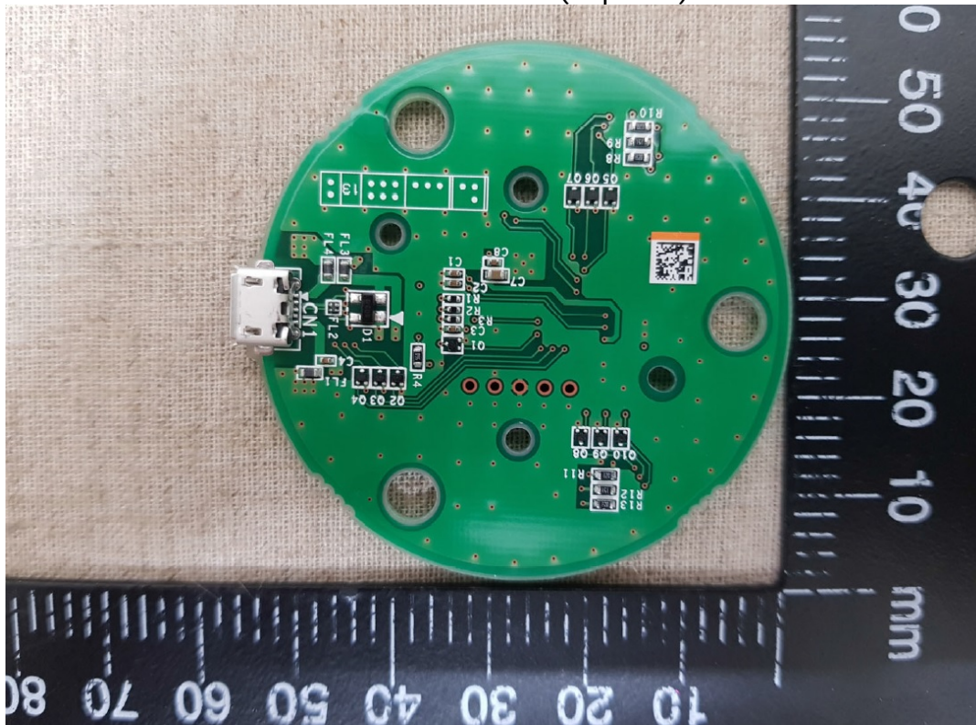
Photo8: CPU Board (Rear side)
