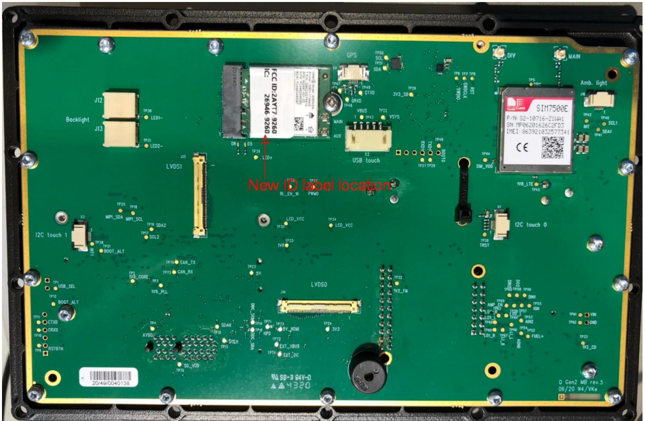
Figure 4 WiFi/BT module new ID label location inside the device
