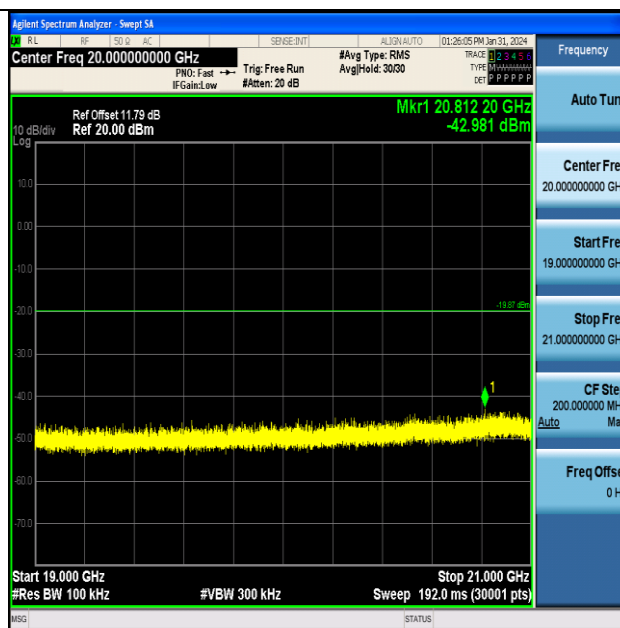
BLE_1M-Ant1-2402-19000~21000-PASS
