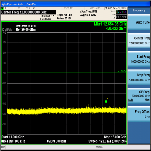
BLE_1M-Ant1-2480-11000~13000-PASS
