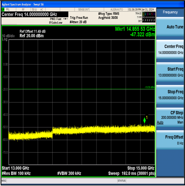
BLE_1M-Ant1-2480-13000~15000-PASS
