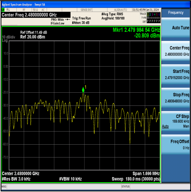
BLE_2M-Ant1-2480-PASS
