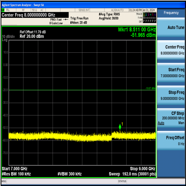
BLE_1M-Ant1-2402-7000~9000-PASS
