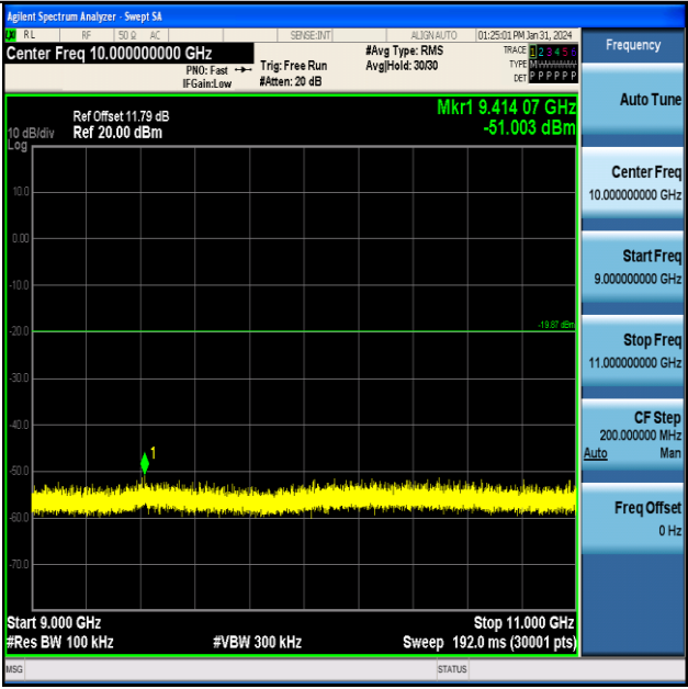
BLE_1M-Ant1-2402-9000~11000-PASS
