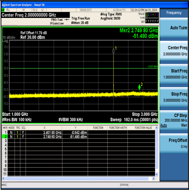
BLE_1M-Ant1-2402-1000~3000-PASS
