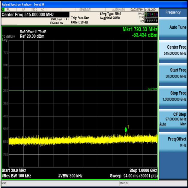
BLE_1M-Ant1-2402-30~1000-PASS
