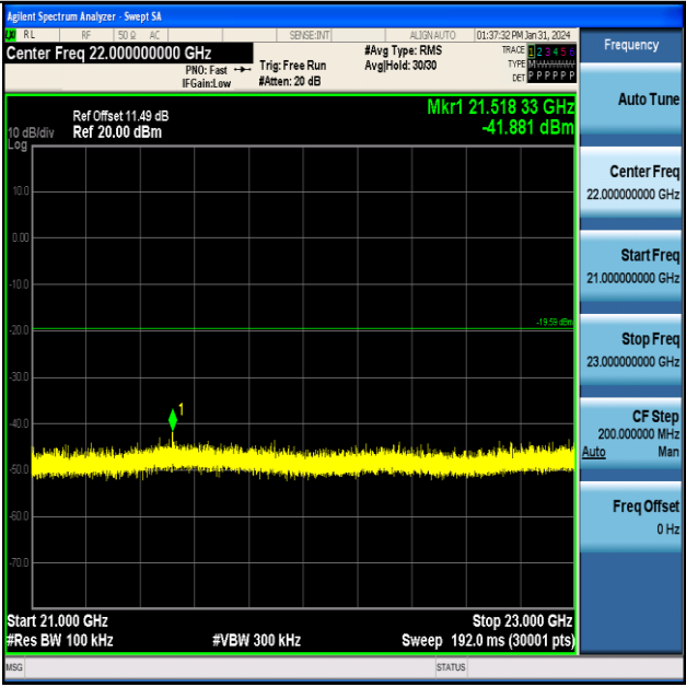
BLE_1M-Ant1-2480-21000~23000-PASS
