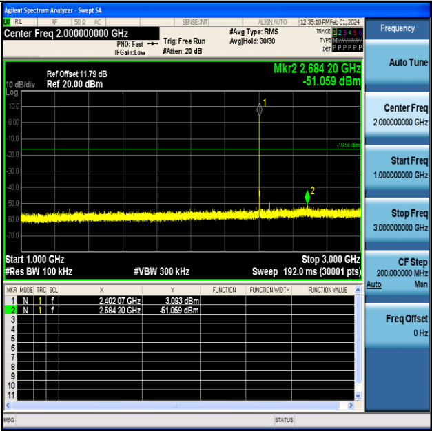
2DH5-Ant1-2402-1000~3000-PASS
