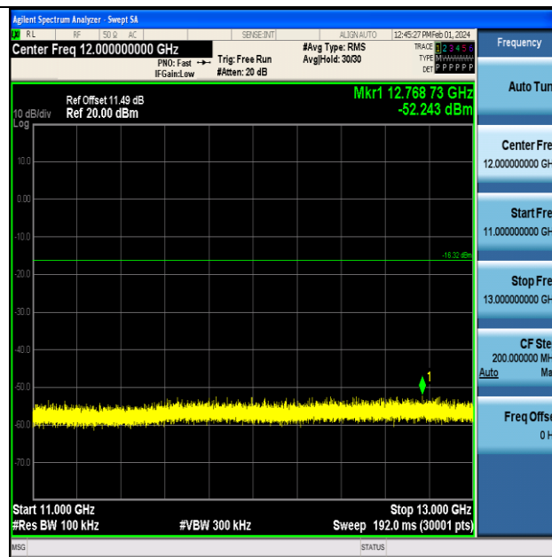
2DH5-Ant1-2480-11000~13000-PASS
