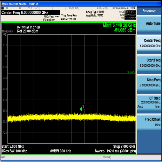
3DH5-Ant1-2441-5000~7000-PASS
