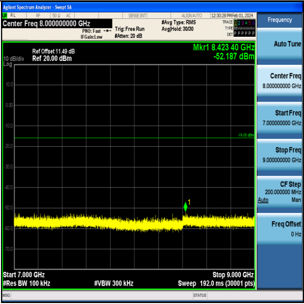
DH5-Ant1-2480-7000~9000-PASS
