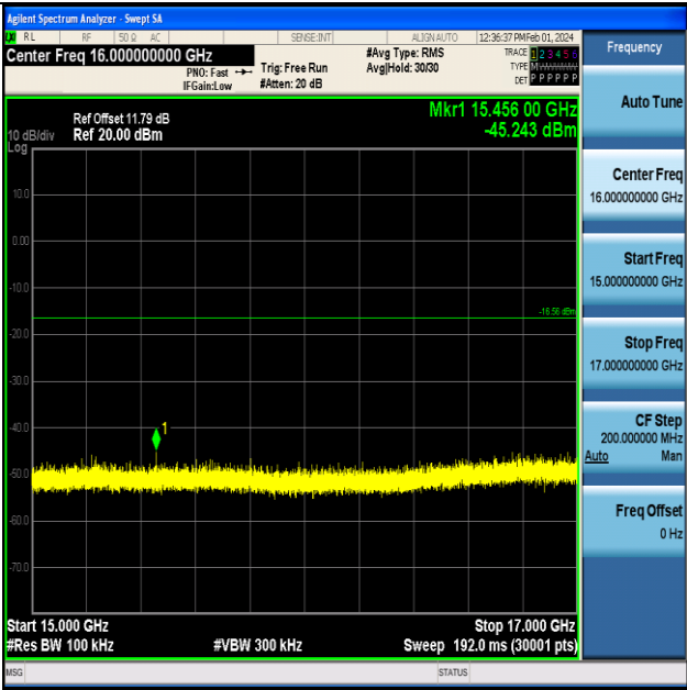
2DH5-Ant1-2402-15000~17000-PASS
