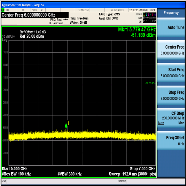
DH5-Ant1-2480-5000~7000-PASS
