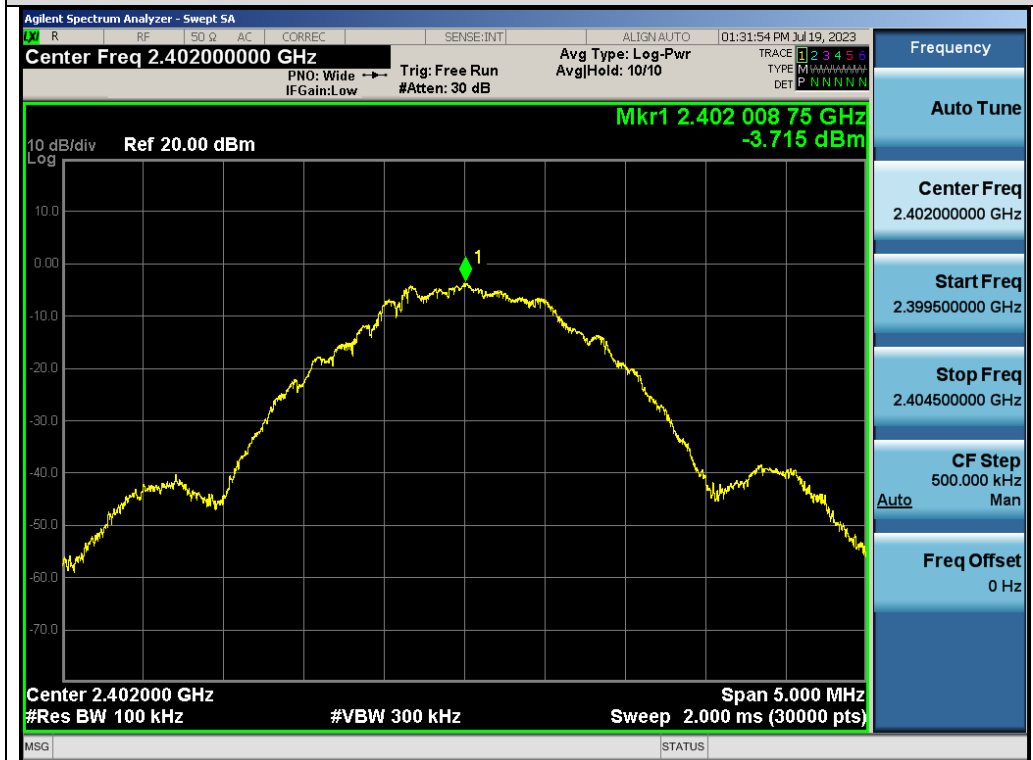
Test_Graph_LE2M_ANT1_2402_2Mbps_Reference Level
