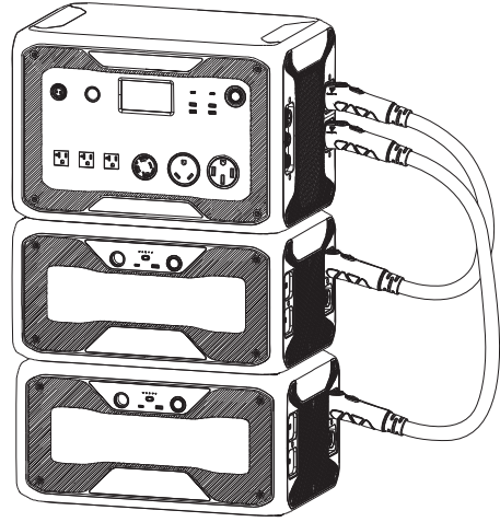
AC500 + 2*B300S = 5000W Max. / 6144Wh
