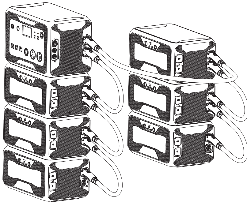
AC500 + 6*B300S = 5000W Max. / 18432Wh
