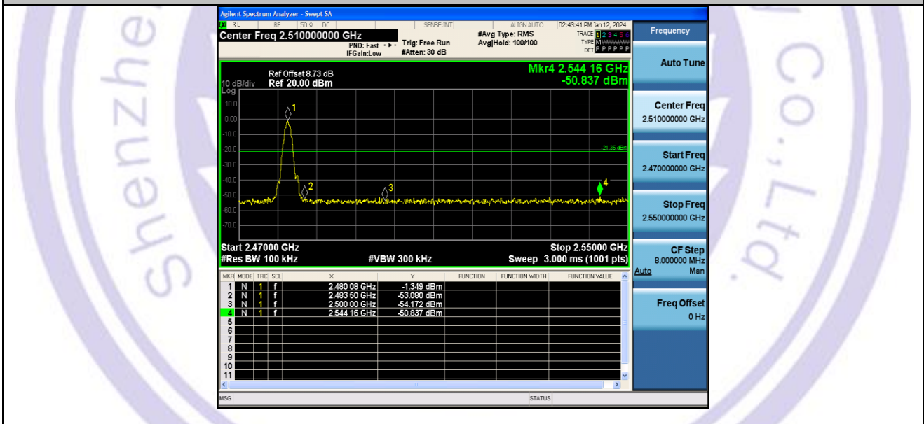
BLE_2M_Ant1_High_2480
