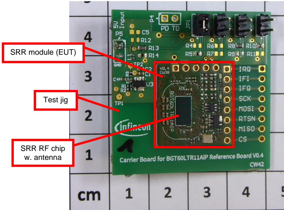
Back view of SRR module (EUT):
