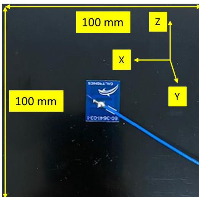
Figure 3 Measurement Orientation
