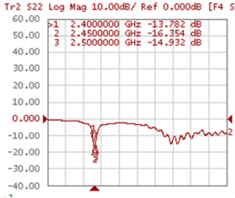
Figure 1 Return Loss
