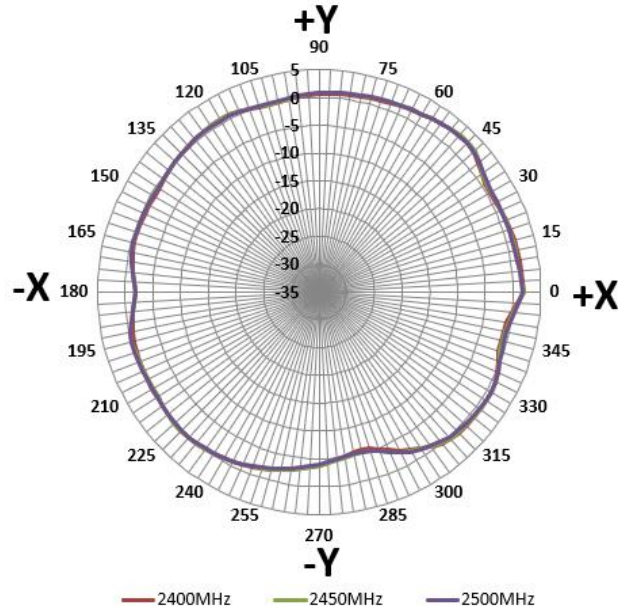
(A). Azimuth plane (XY plane) radiation pattern
