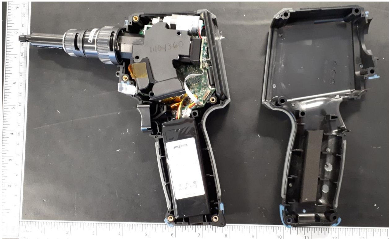
Interior View of top enclosure with internal battery removed.
