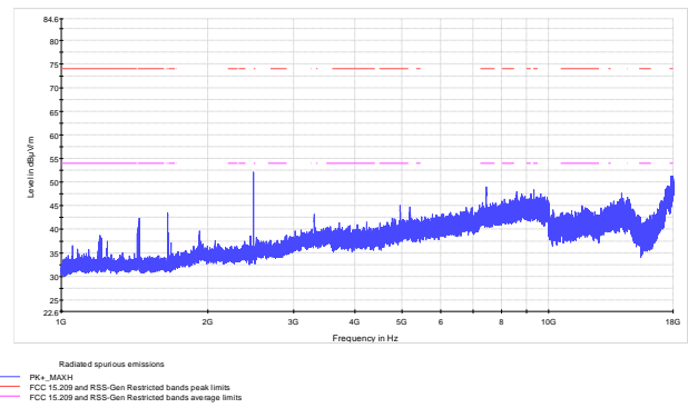
Figure 8.5-8: Radiated spurious emissions within 1–18 GHz, top channel
