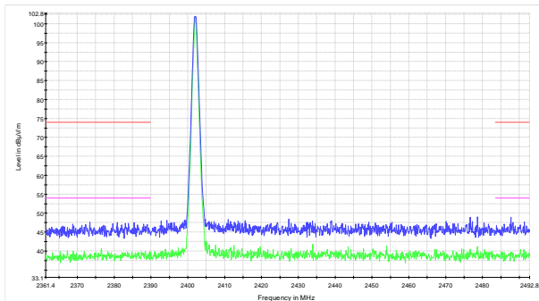
Figure 8.5-1: Band edge spurious emissions at 2400 MHz
