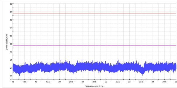
Radiated spurious emissions PK+, MAXH FCC Part 15 and ICES-003 Limit - Class B (PK) above 1 GHz, 3 m FCC Part 15 and ICES-003 Limit - Class B (DP and Avg), 3 m
