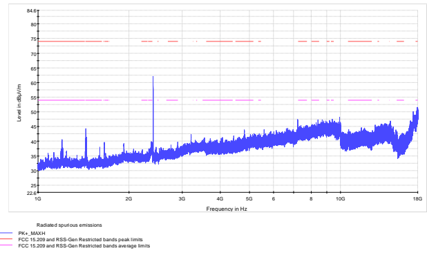
Figure 8.5-6: Radiated spurious emissions within 1–18 GHz, low channel
