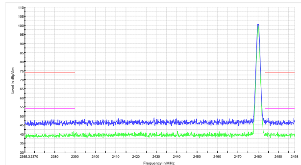
Figure 8.5-2: Band edge spurious emissions at 2483.5 MHz
