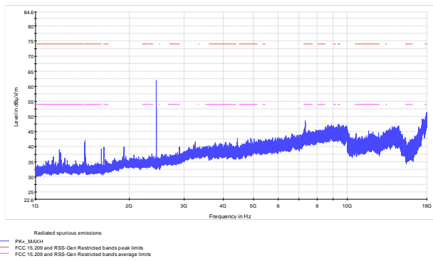
Figure 8.5-7: Radiated spurious emissions within 1–18 GHz, mid channel
