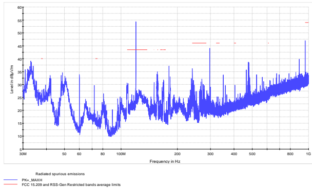
Figure 8.5-3: Radiated spurious emissions within 30–1000 MHz, low channel
