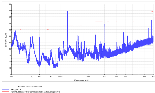
Figure 8.5-5: Radiated spurious emissions within 30–1000 MHz, top channel
