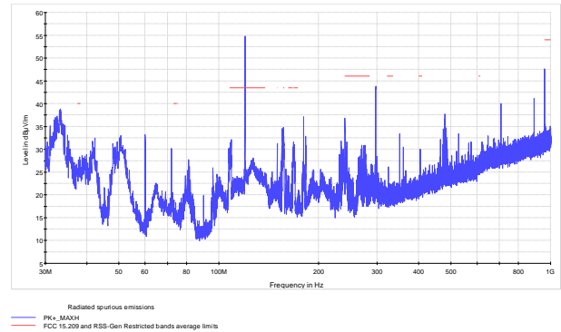
Figure 8.5-4: Radiated spurious emissions within 30–1000 MHz, mid channel
