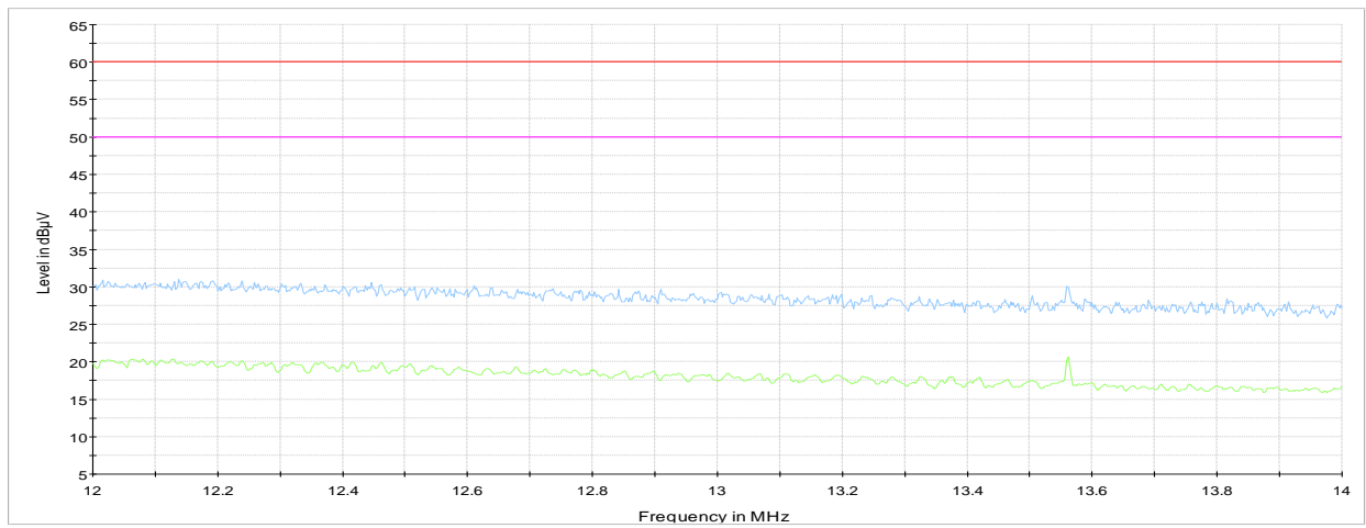
Conducted emissions on Neutral line (around 13 MHz)
