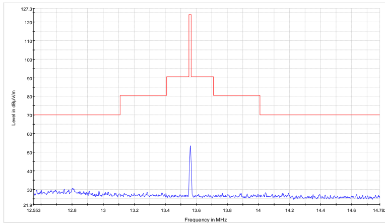
Figure 8.6-3: Field strength within 13.110–14.010 MHz band
