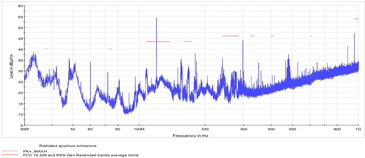
Figure 8.7-2: Field strength of spurious emissions above 30 MHz
