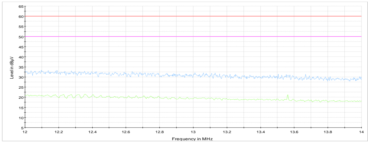
Conducted emissions on Phase line (around 13 MHz)
