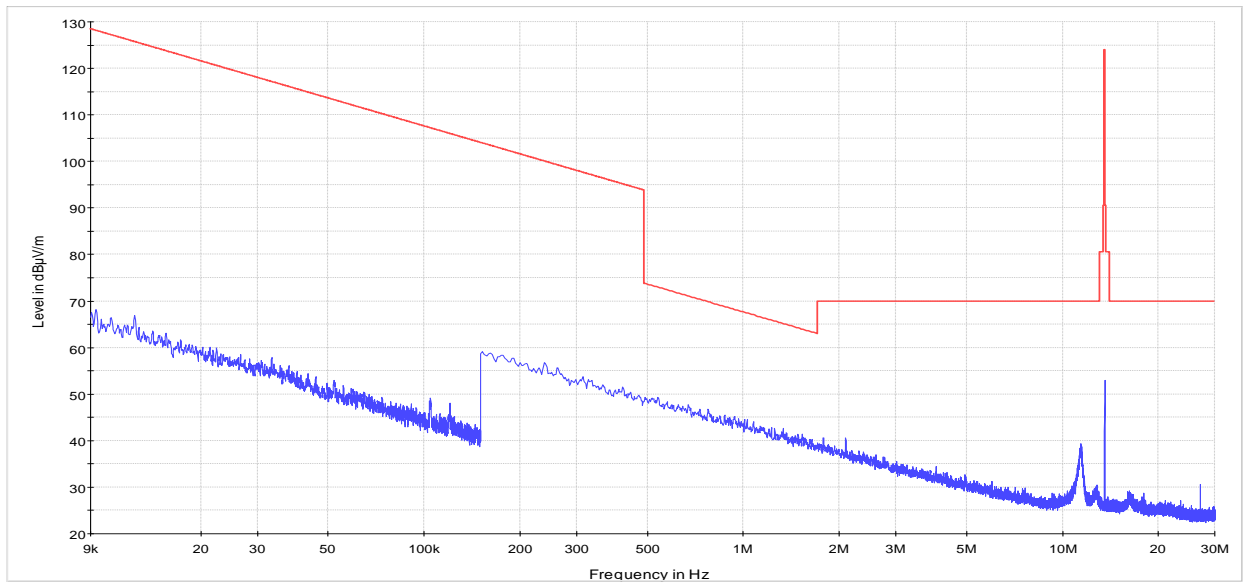
Figure 8.7-1: Field strength of spurious emissions below 30 MHz
