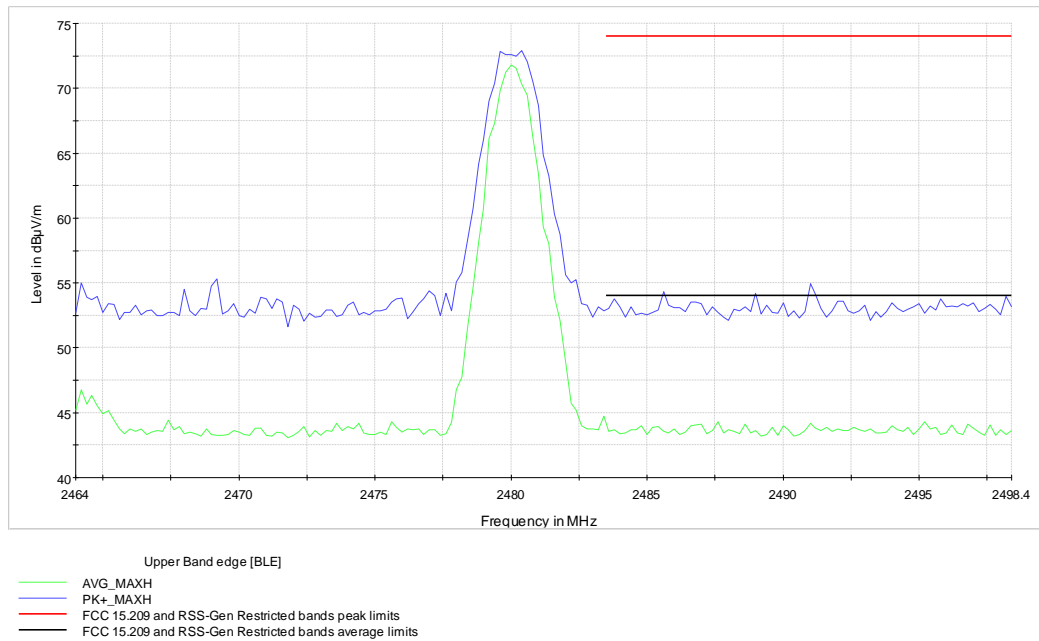
Figure 7.2-4: Radiated spurious emissions on upper band edge [BLE]
