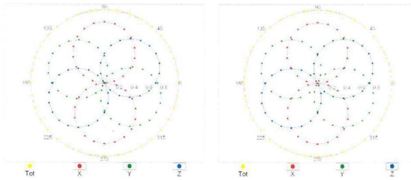
f=600 MHz,TEM
