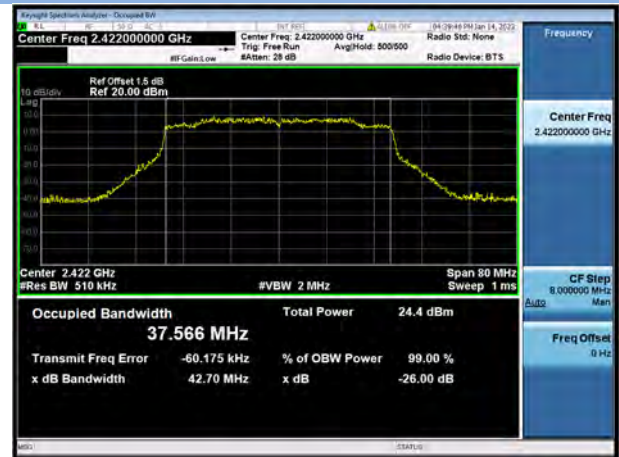
802.11ax-40 MHz(SU) CHANNEL 3
