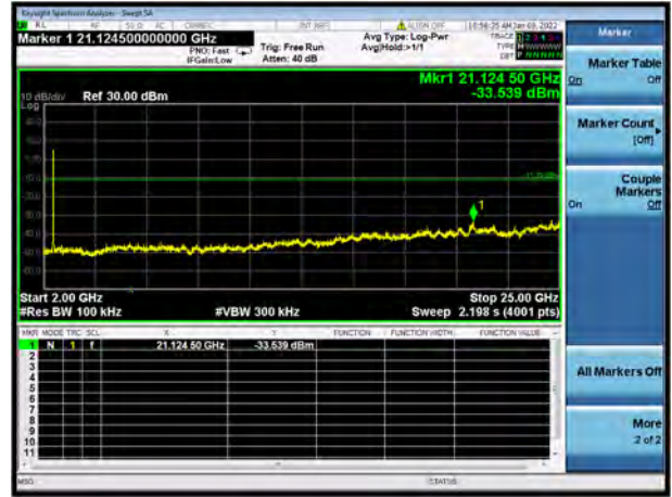
802.11ax-20 MHz(SU) MIDDLE CHANNEL, SPURIOUS 2 GHz ~ 25 GHz
