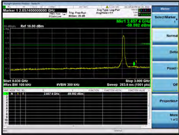
802.11ax-40 MHz(SU) MIDDLE CHANNEL, SPURIOUS 30 MHz ~ 3 GHz
