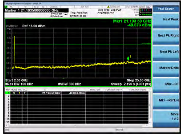
802.11ax-40 MHz(SU) MIDDLE CHANNEL, SPURIOUS 2 GHz ~ 25 GHz
