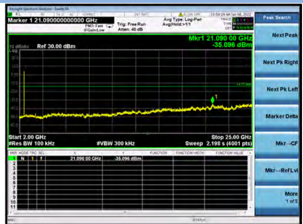
802.11ax-20 MHz(SU) HIGH CHANNEL, SPURIOUS 2 GHz ~ 25 GHz
