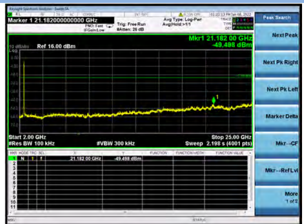
802.11ax-40 MHz(SU) HIGH CHANNEL, SPURIOUS 2 GHz ~ 25 GHz
