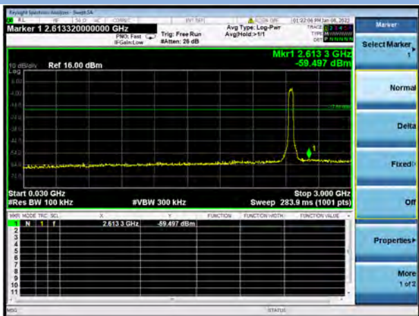
802.11ax-40 MHz(SU) HIGH CHANNEL, SPURIOUS 30 MHz ~ 3 GHz
