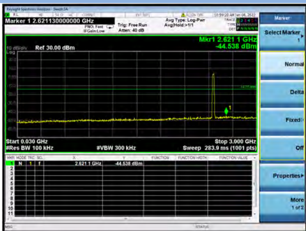
802.11ax-20 MHz(SU) HIGH CHANNEL, SPURIOUS 30 MHz ~ 3 GHz
