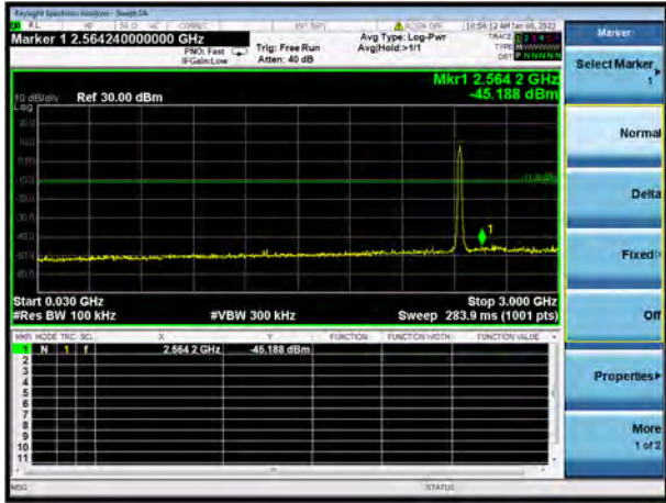
802.11ax-20 MHz(SU) MIDDLE CHANNEL, SPURIOUS 30 MHz ~ 3 GHz
