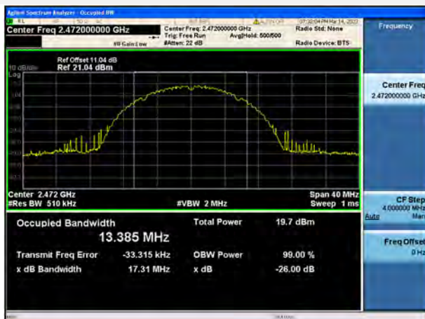
802.11b CHANNEL 13
