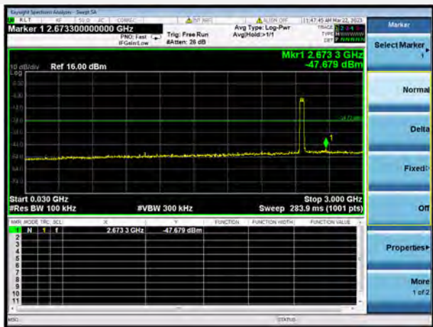
802.11n-40 MHz CHANNEL 11, SPURIOUS 30 MHz ~ 3 GHz
