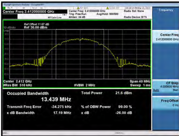
802.11b CHANNEL 1
