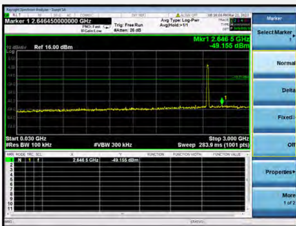
802.11ax-20 MHz(SU) CHANNEL 12, SPURIOUS 30 MHz ~ 3 GHz
