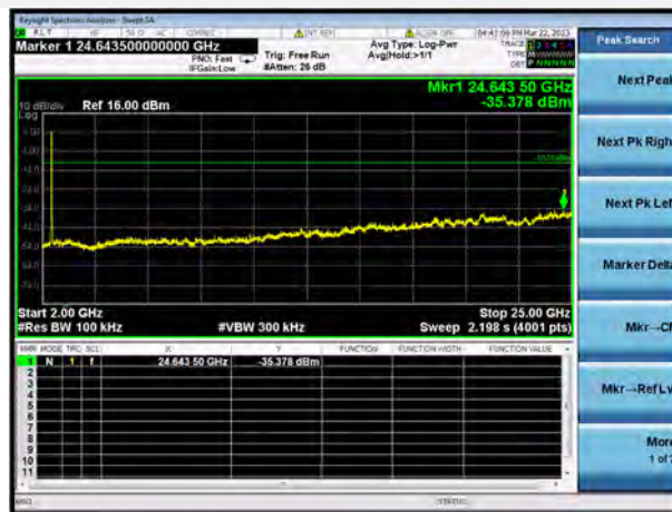
802.11ax-20 MHz(SU) CHANNEL 1, SPURIOUS 2 GHz ~ 25 GHz
