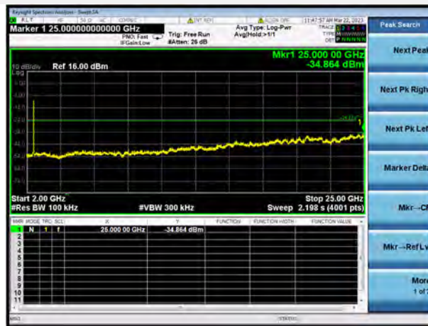
802.11n-40 MHz CHANNEL 11, SPURIOUS 2 GHz ~ 25 GHz
