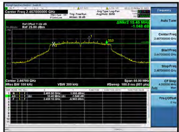
802.11n-20 MHz CHANNEL 12
