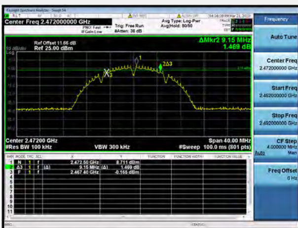
802.11b CHANNEL 13
