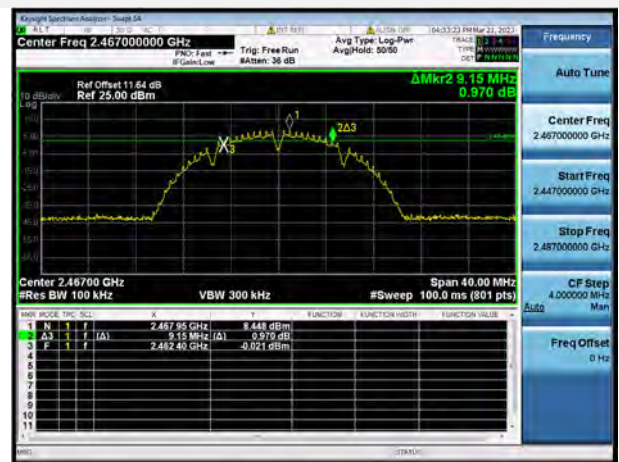
802.11b CHANNEL 12
