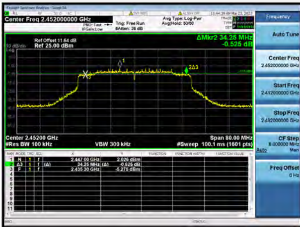
802.11ax-40 MHz(SU) CHANNEL 9
