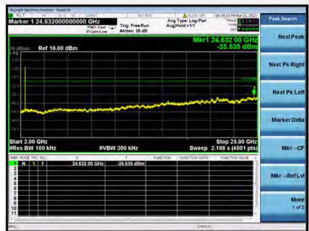
802.11ax-20 MHz(SU) CHANNEL 12, SPURIOUS 2 GHz ~ 25 GHz
