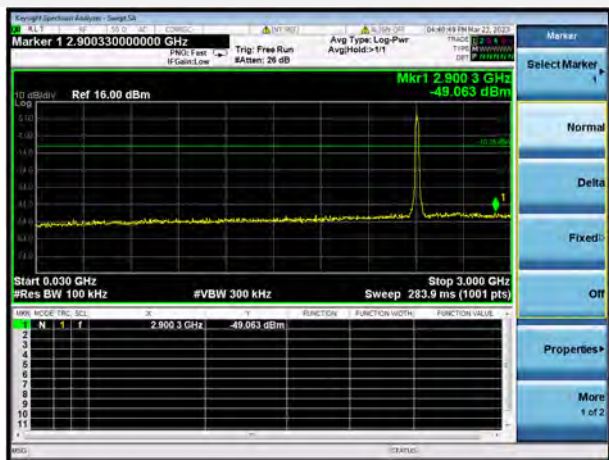
802.11ax-20 MHz(SU) CHANNEL 1, SPURIOUS 30 MHz ~ 3 GHz
