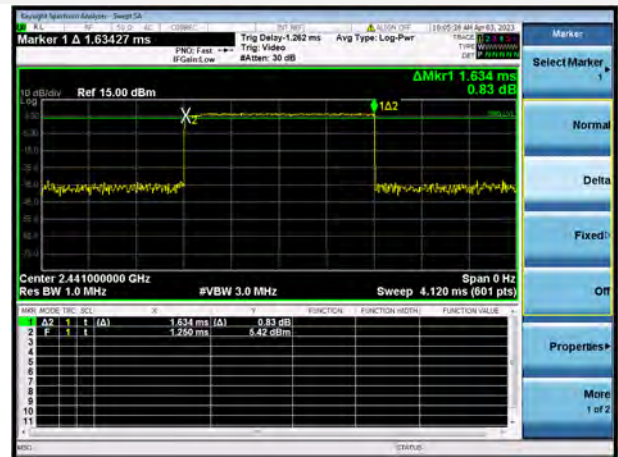
8-DPSK DH3
