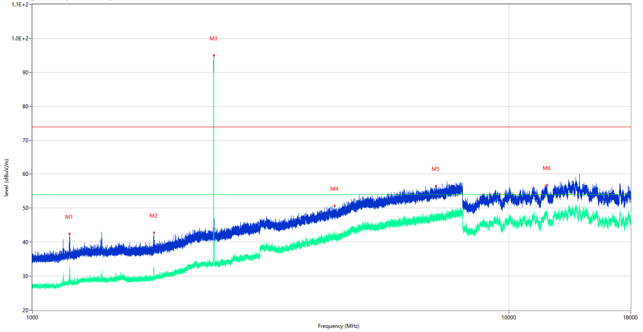
RE Test case_FCC Part 15C_FCC 15.247(2.4G)_1GHz-18GHz
