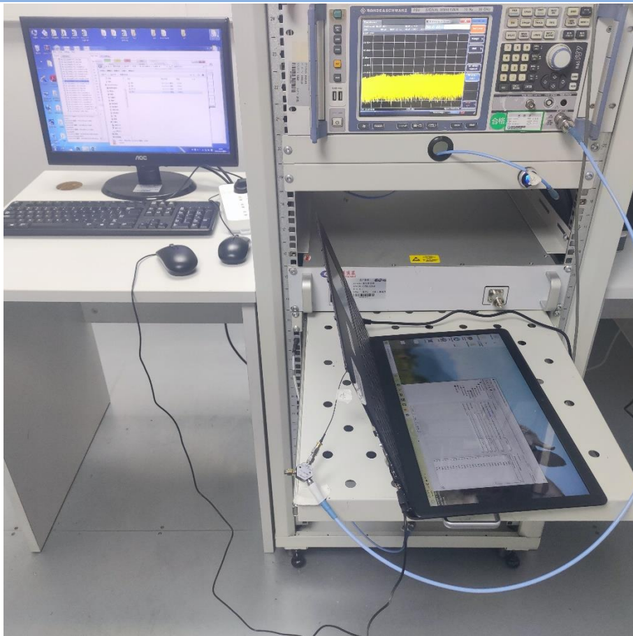
Conducted Test-BT3.0
