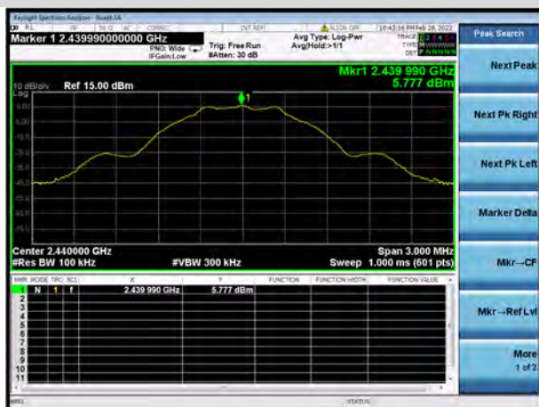
GFSK (BLE 1Mbps) MIDDLE CHANNEL, CARRIER LEVEL
