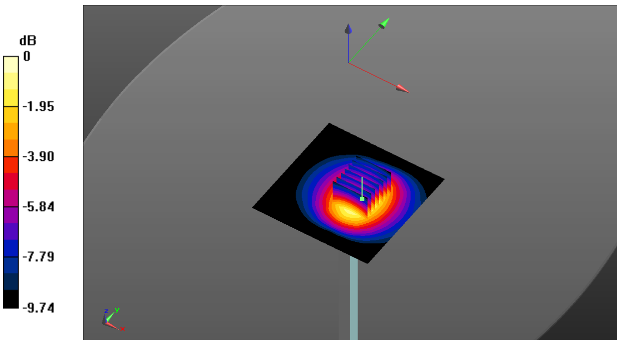
0 dB = 0.916 W/kg
