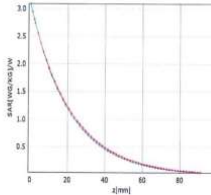
~ analytical ~ measured
