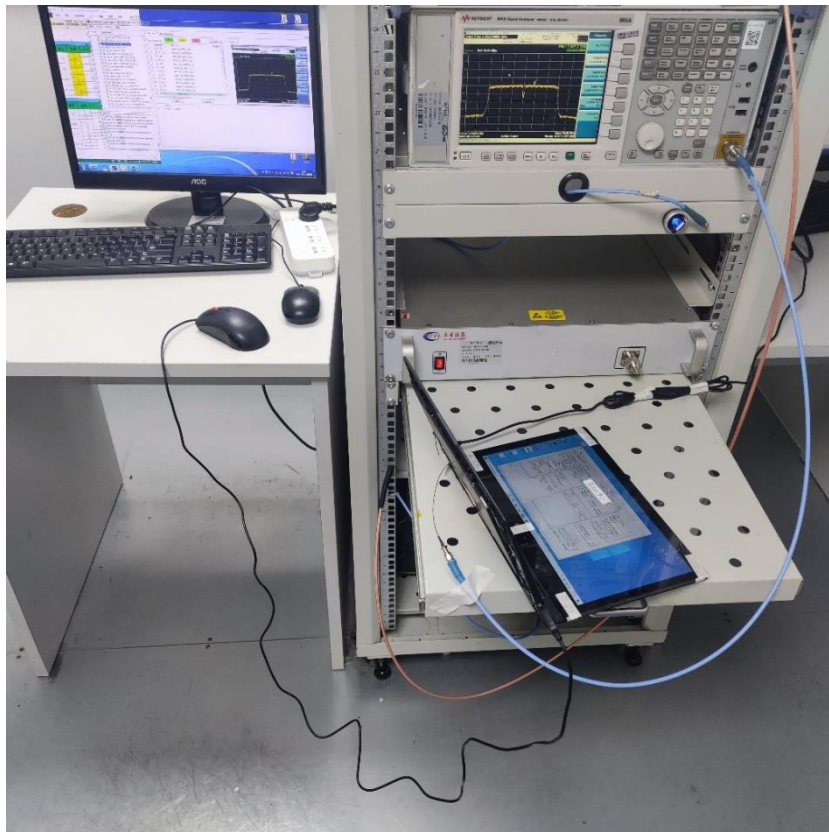
Conducted Test-2.4G WIFI
