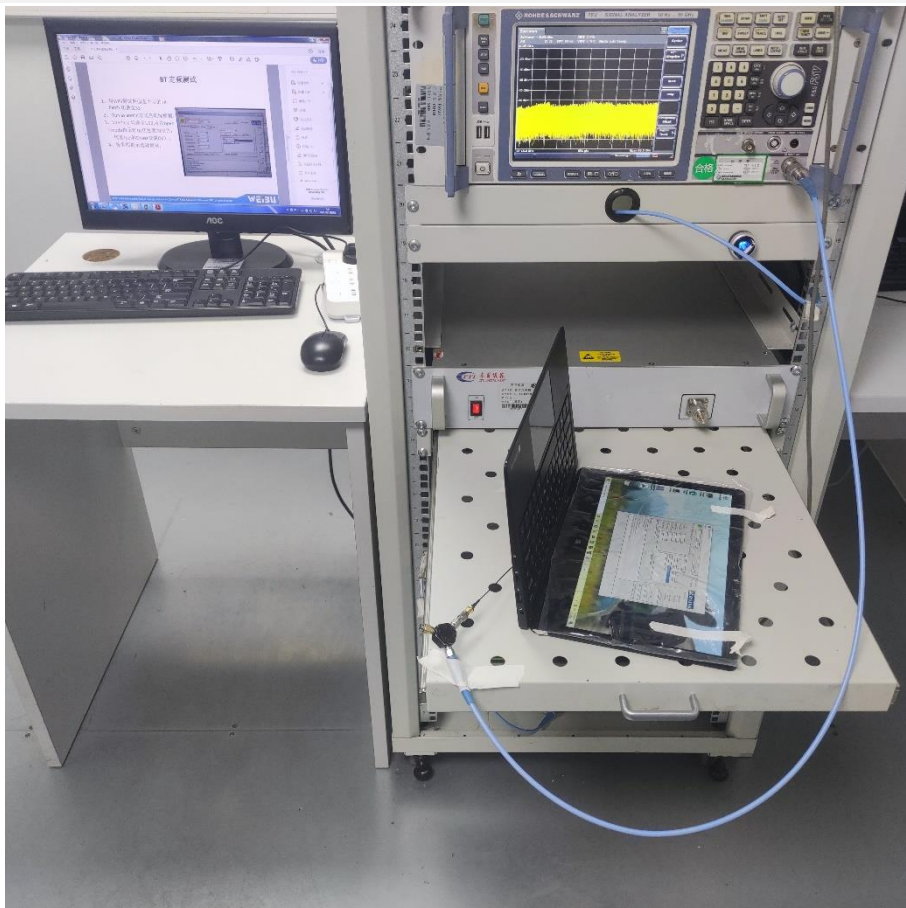
Conducted Test-BT
