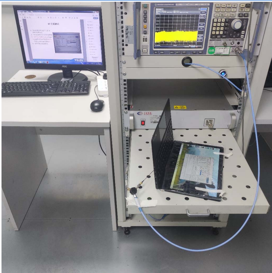
Conducted Test-BT3.0/BLE
