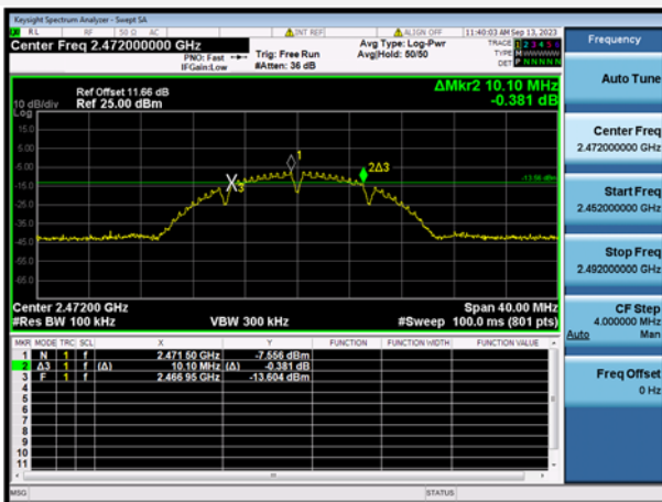
802.11b CHANNEL 13
