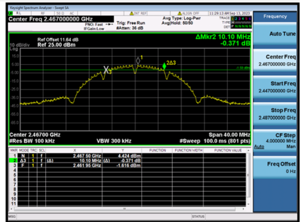
802.11b CHANNEL 12
