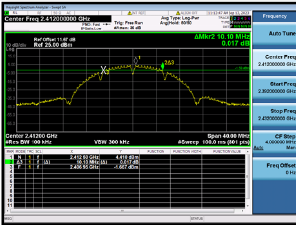
802.11b CHANNEL 1
