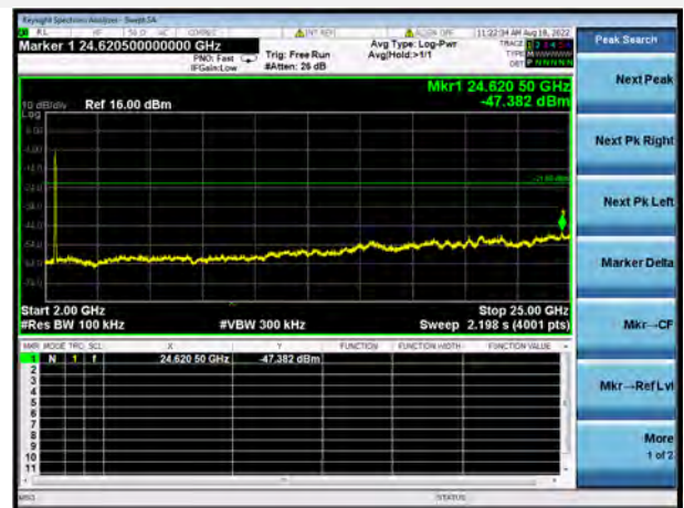
802.11n-40 MHz HIGH CHANNEL, SPURIOUS 2 GHz ~ 25 GHz
