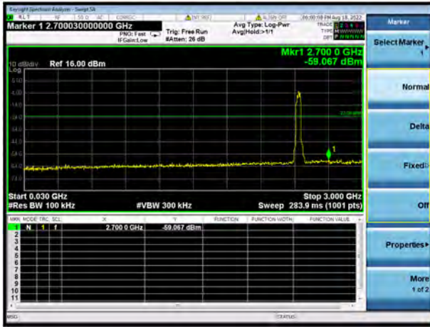
802.11n-40 MHz MIDDLE CHANNEL, SPURIOUS 30 MHz ~ 3 GHz
