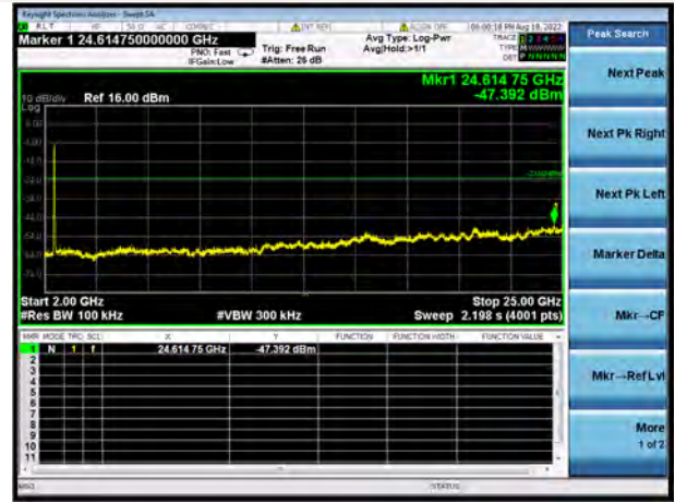
802.11n-40 MHz MIDDLE CHANNEL, SPURIOUS 2 GHz ~ 25 GHz
