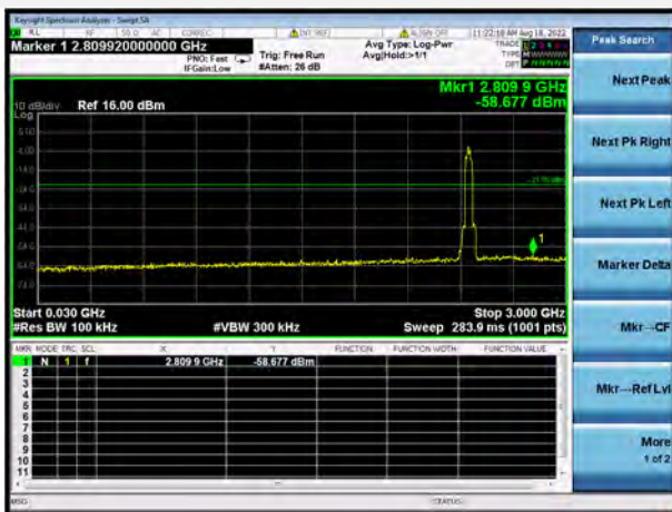
802.11n-40 MHz HIGH CHANNEL, SPURIOUS 30 MHz ~ 3 GHz
