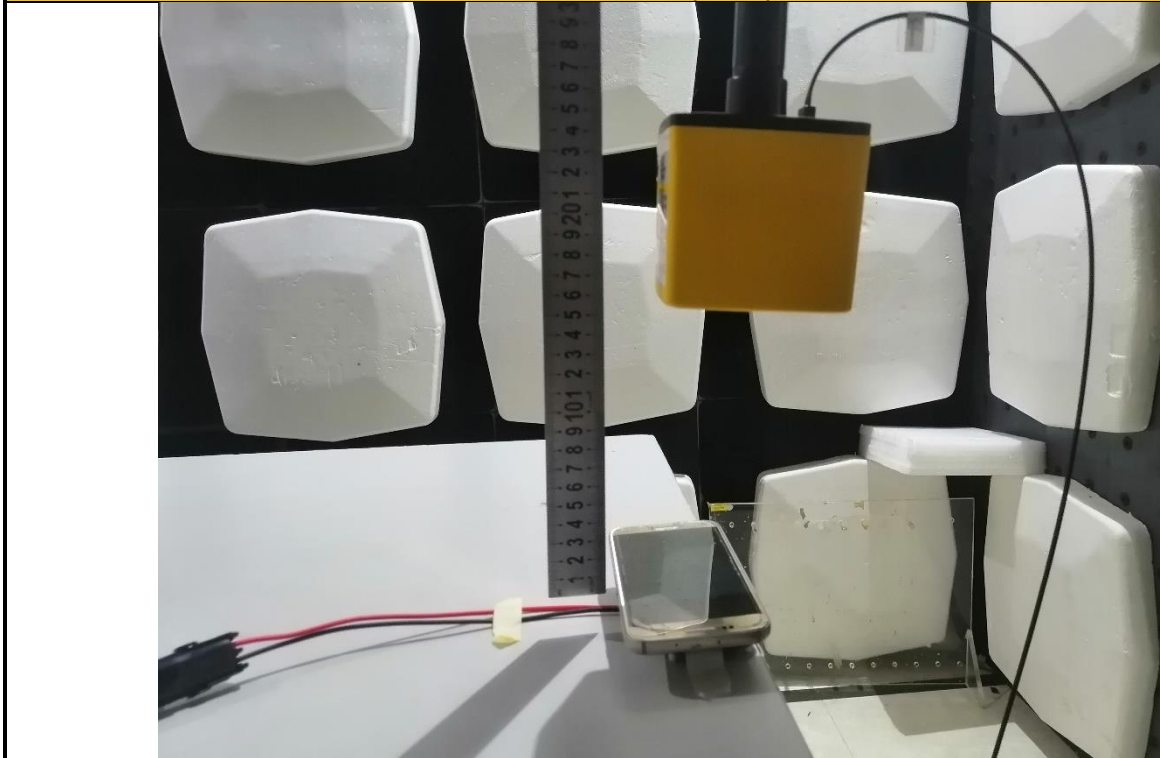
E-Field Strength and H-Field Strength Position E (20cm)
