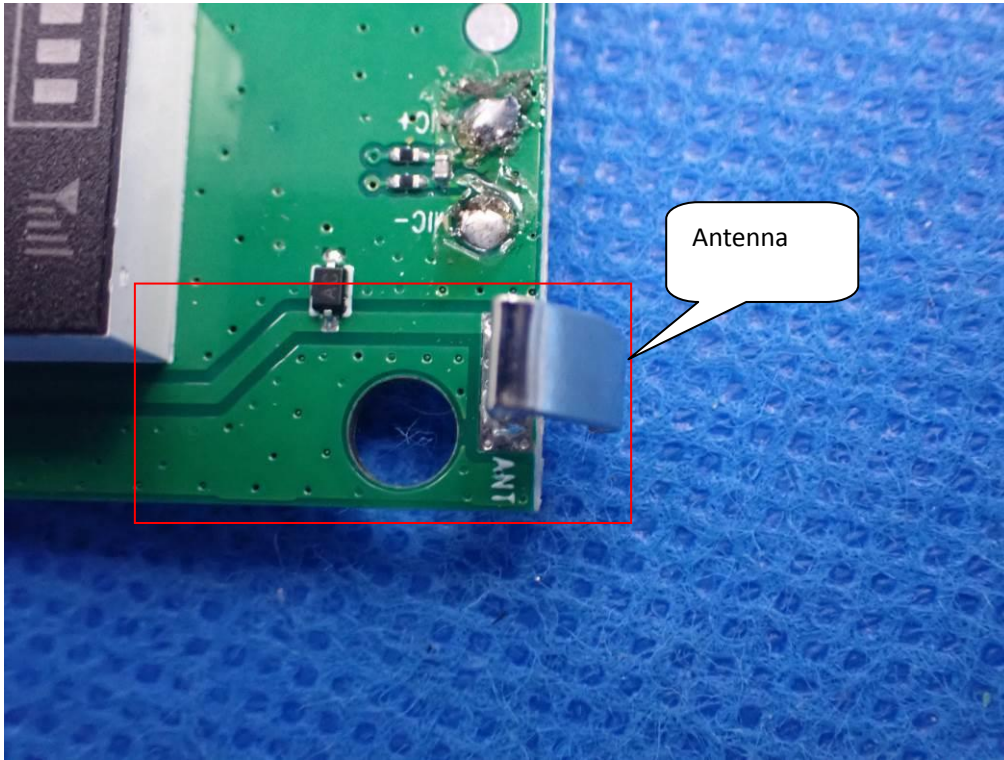
INTERNAL VIEW-5 OF Microphone
