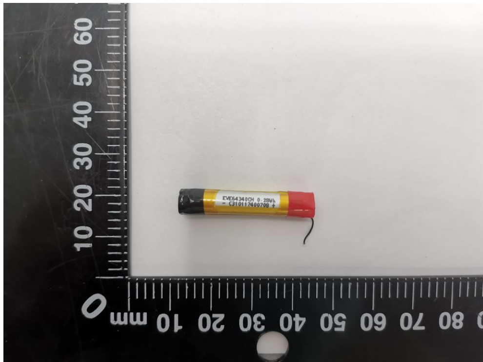
Fig.8 Battery view
