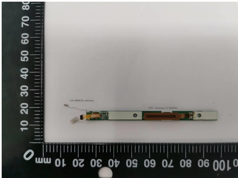
Fig.6 PCB view-01
