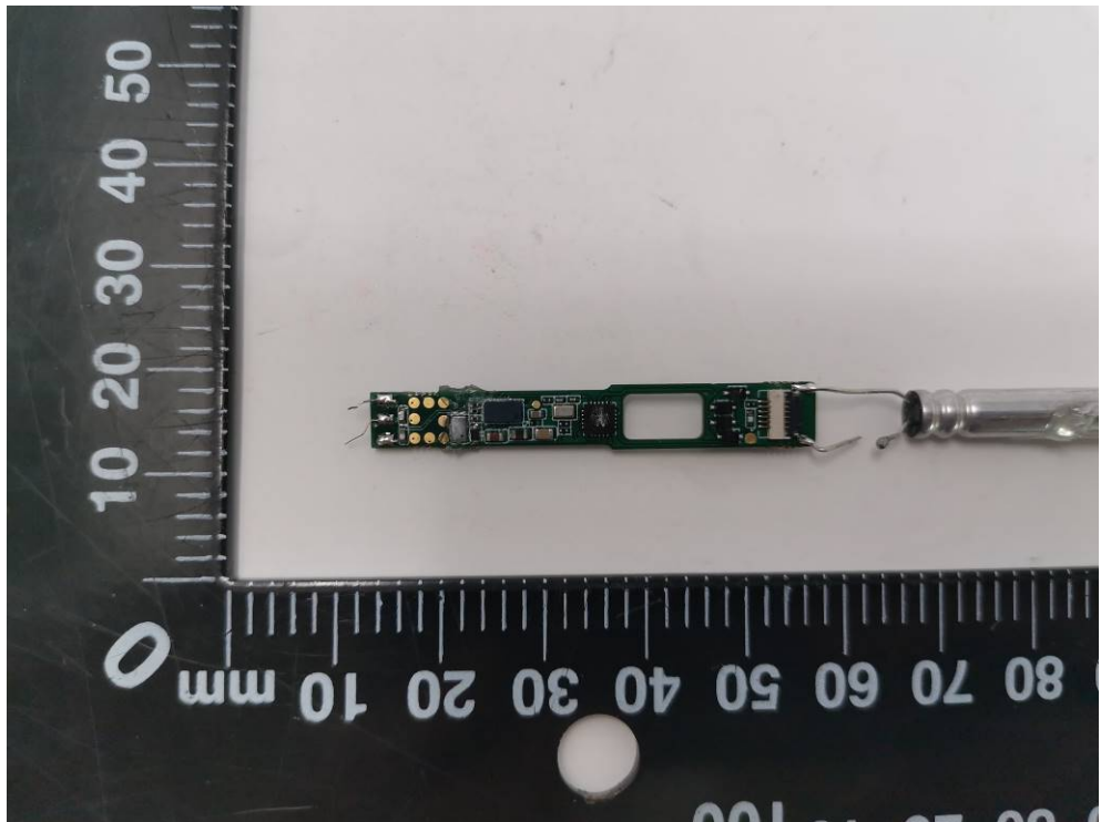
Fig.4 PCB view-02
