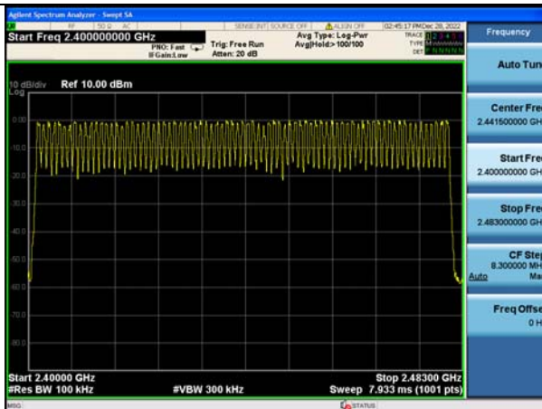
GFSK Modulation
