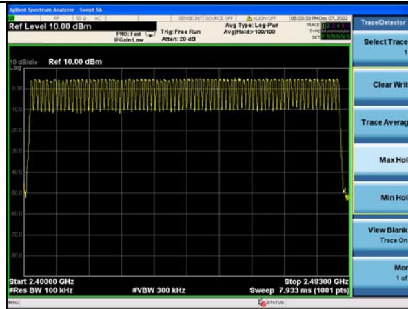
GFSK Modulation
