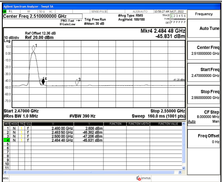
3DH5_Ant1_High_2480_Peak
