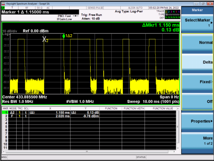
(Time per burst: 1.150ms*11pcs)
