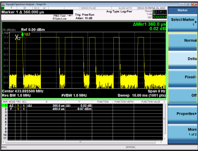
(Time per burst: 0.360ms*14pcs)
