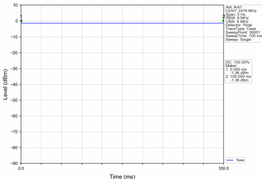
2M_HCH_2478MHz_Ant1_NTNV
