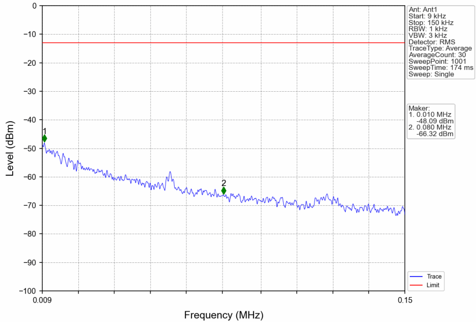
Band4_1.4MHz_16QAM_HCH_1754.3MHz_RB_1_0_NTNV
