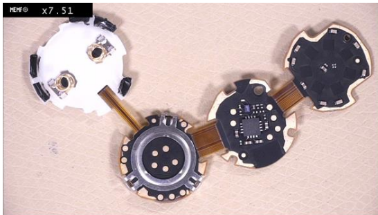
Unfolded PCB- top view
