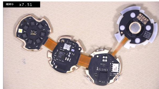
Unfolded PCB- bottom view
