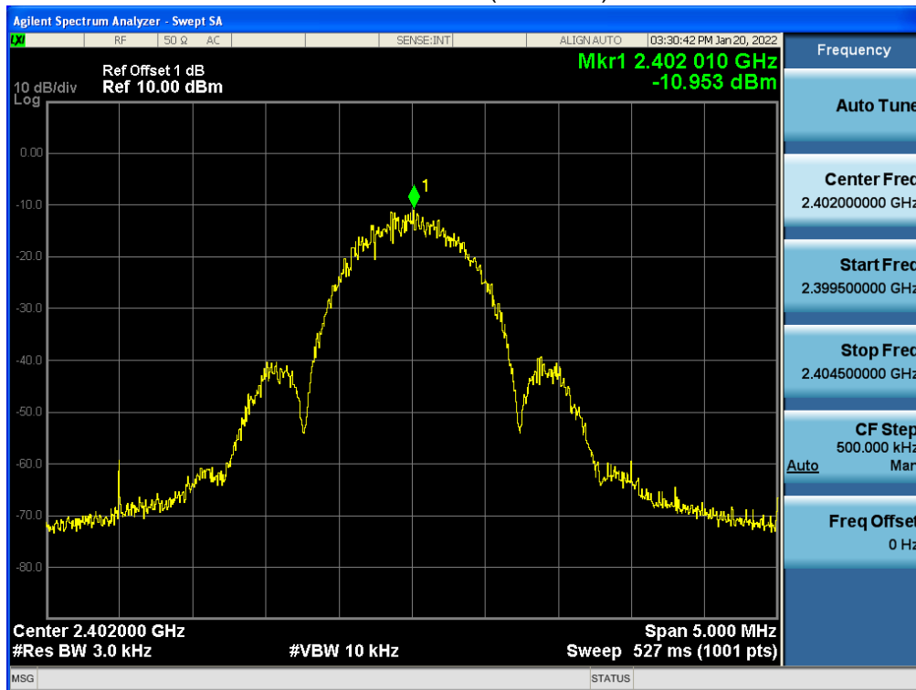
Mode 1 / CH37(2402MHz)
