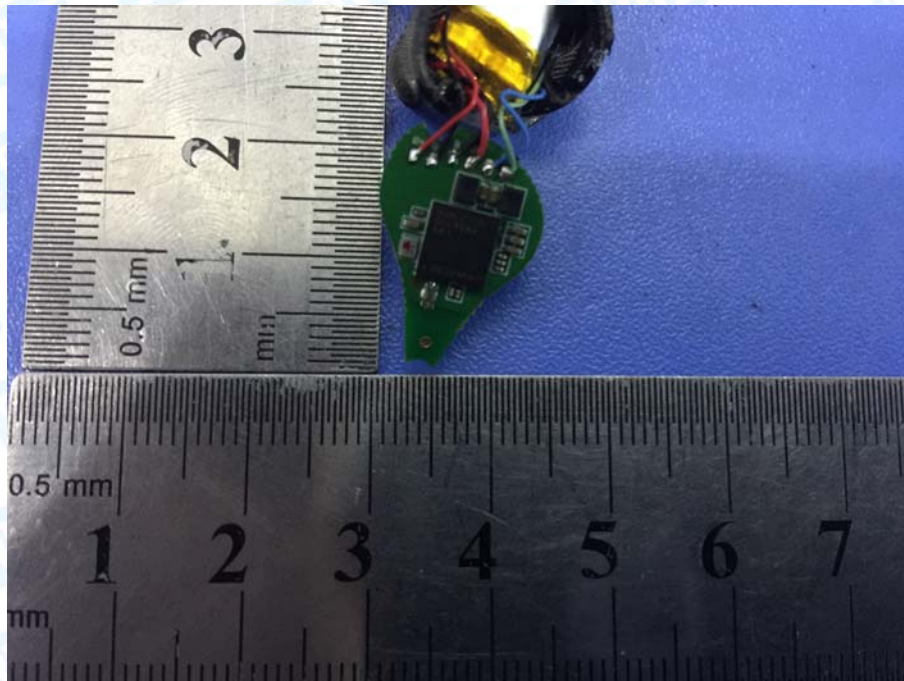
Photo 16 Appearance PCB
